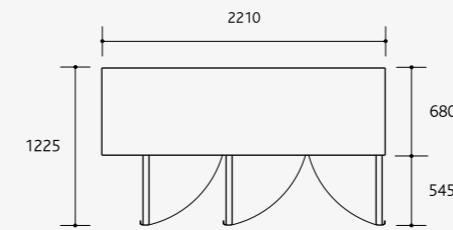
Integral top view
