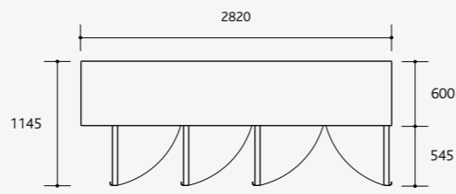
CC700 integral top view
