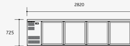
Integral front elevation
