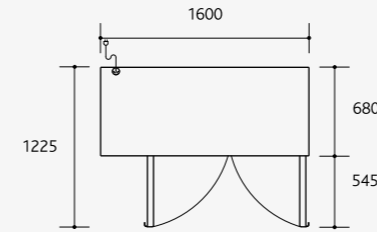
Integral top view
