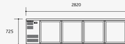
CC700 integral front elevation
