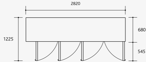
Integral top view
