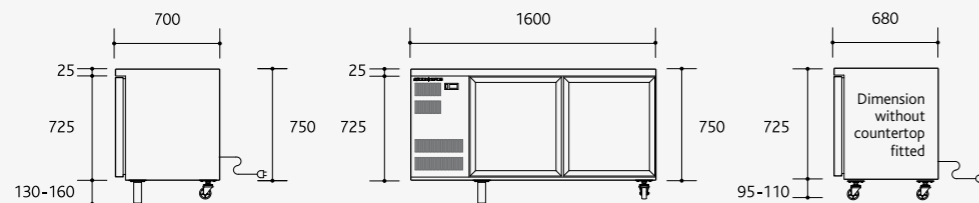
Drawing Depicts: CL400 2SW integral with optional mounting heights Optional countertop height 25mm. Countertop fascia height 65mm. Adjustable front locking swivel castors (95-110mm high) – total height 820-835mm without countertop. Adjustable legs (130-160mm high) – total height 855-885mm without countertop.
