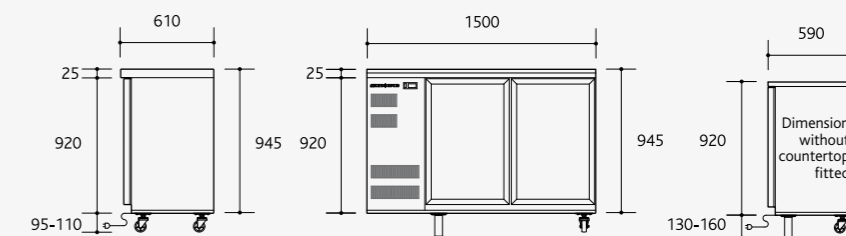
Drawing Depicts: BB380 2SW integral with optional mounting heights Optional countertop height 25mm. Adjustable front locking swivel castors (95-110mm high) – total height 1015-1030mm without countertop. Adjustable legs (130-160mm high) – total height 1050-1080mm without countertop.
